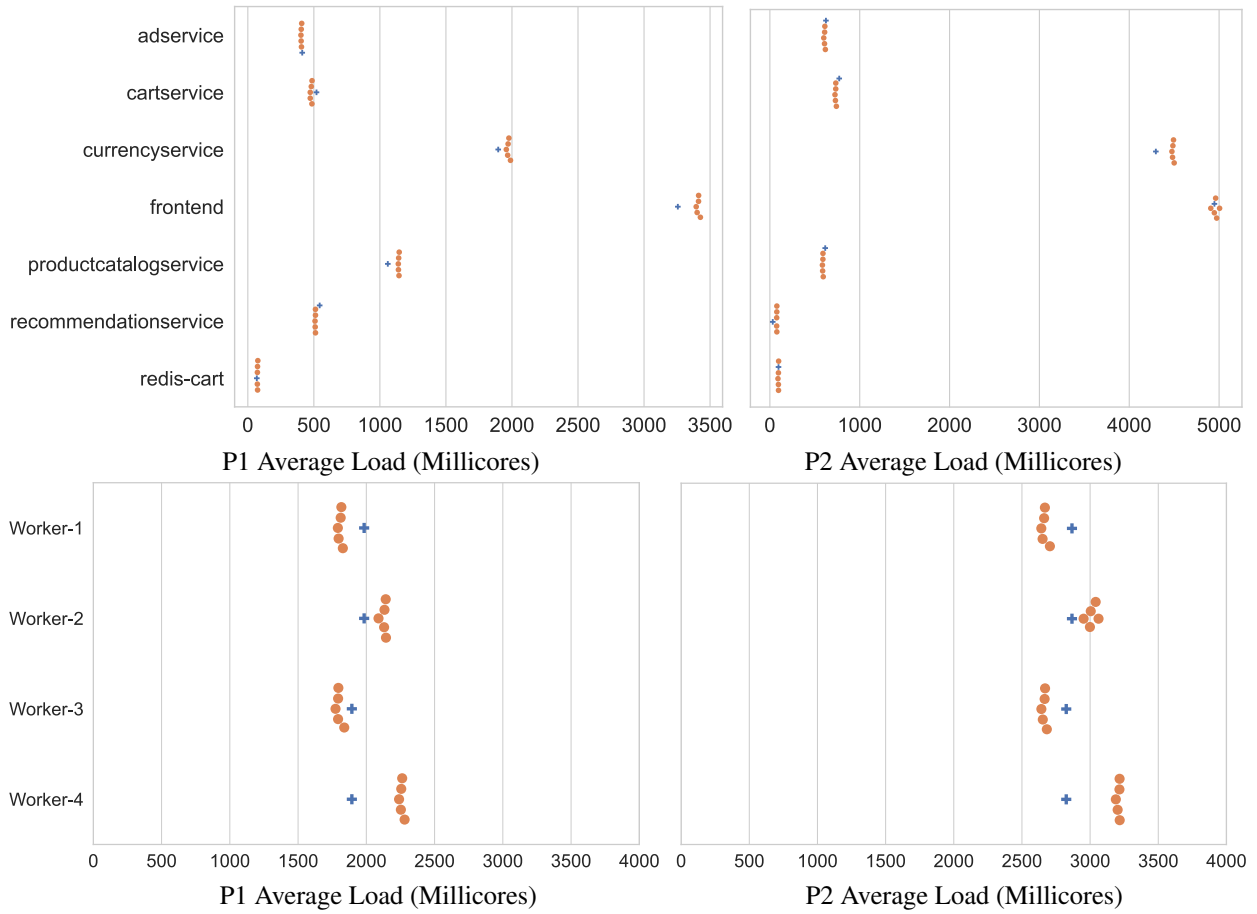
Figure 11: Measurements for the mixed workflows P1 and P2, comparing the resource consumption recorded in the cluster stress tests (orange dots) with the expected values given by the resource model (blue plus). The plots are reported by service (top), and by node (bottom).
