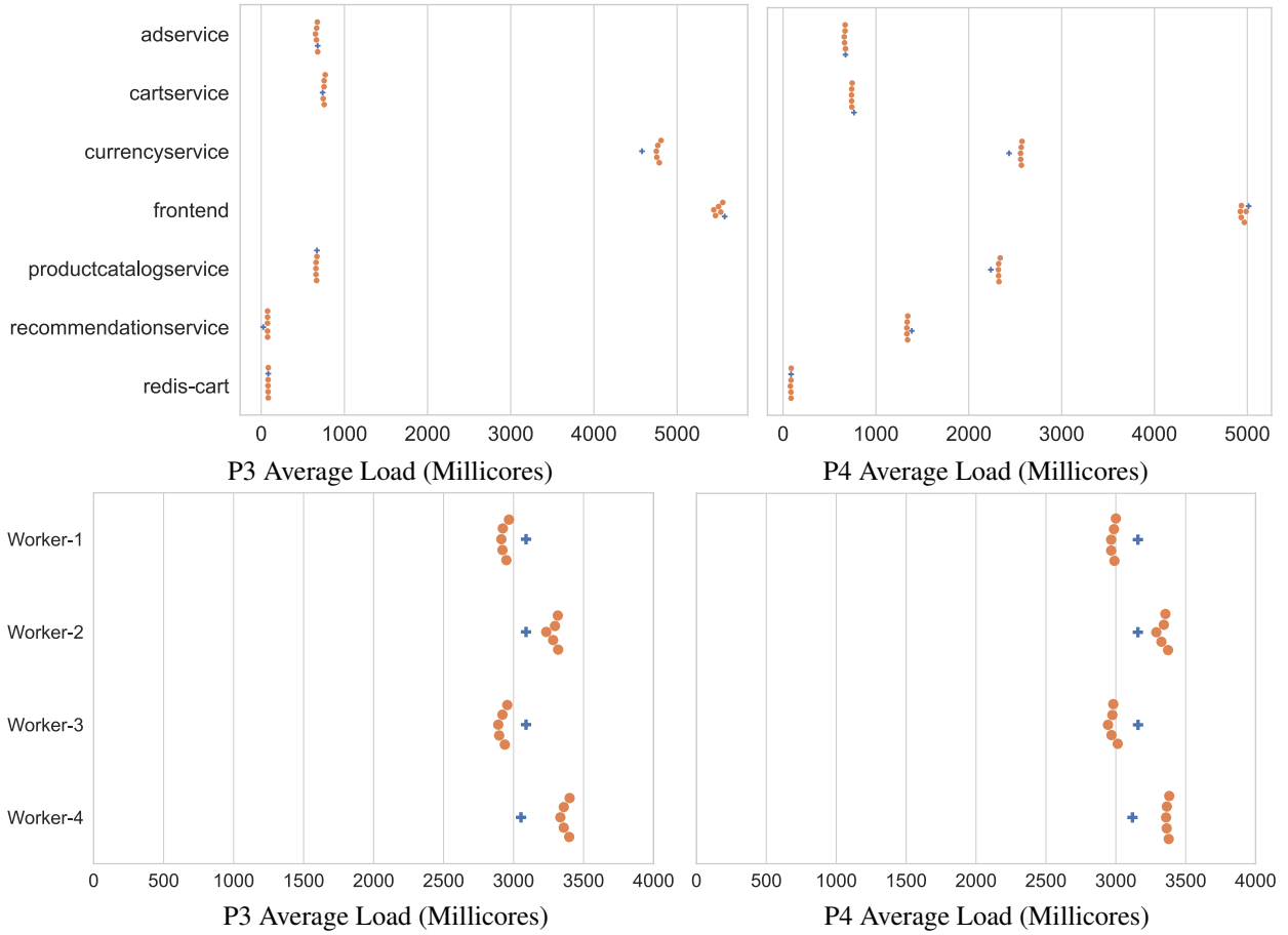
Figure 12: Measurements for the mixed workflows P3 and P4, comparing the resource consumption recorded in the cluster stress tests (orange dots) with the expected values given by the resource model (blue plus). The plots are reported by service (top), and by node (bottom).
