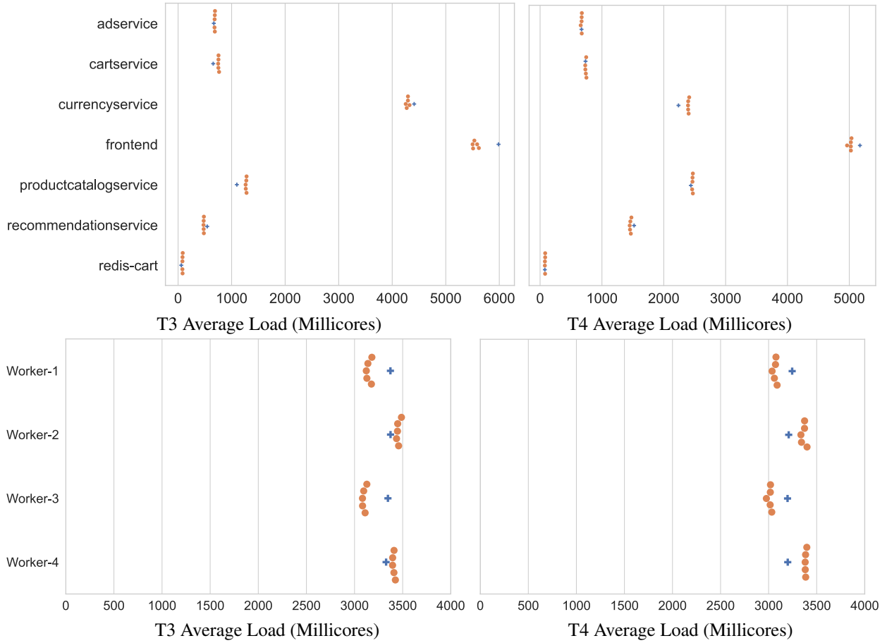
Figure 14: Measurements for the mixed workflows T3 and T4, comparing the resource consumption recorded in the cluster stress tests (orange dots) with the expected values given by the resource model (blue plus). The plots are reported by service (top), and by node (bottom).
