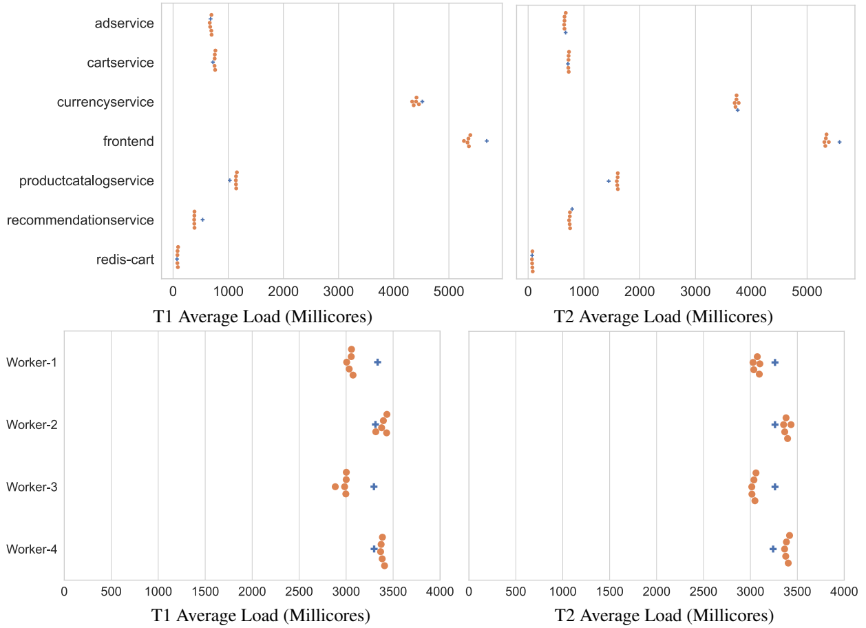
Figure 13: Measurements for the mixed workflows T1 and T2, comparing the resource consumption recorded in the cluster stress tests (orange dots) with the expected values given by the resource model (blue plus). The plots are reported by service (top), and by node (bottom).
