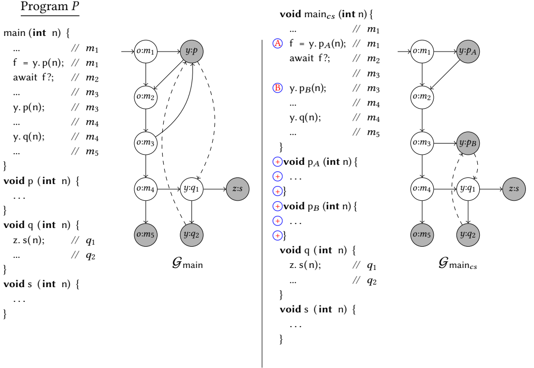
Fig. 7. Context-sensitive example
