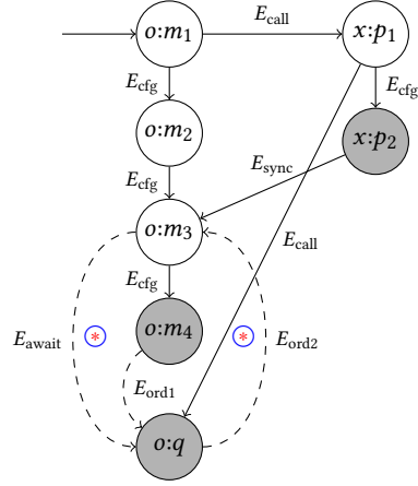
Fig. 4. DFG of a program with cooperative concurrency
