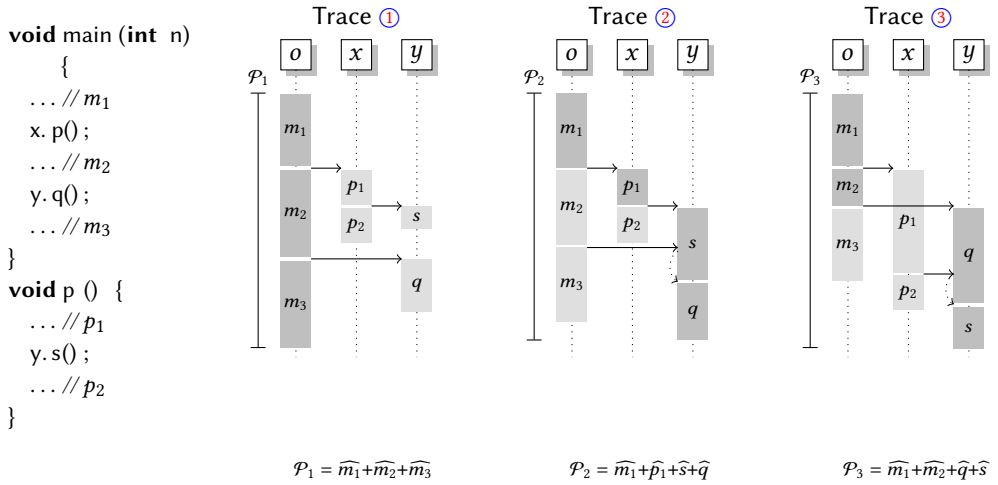
Fig. 2. Motivating example
